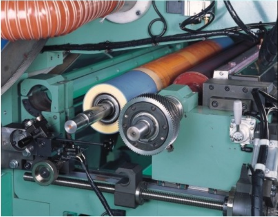
Plate cylinder by sleeve quick change system 版輪採用套筒式快速更換系統
